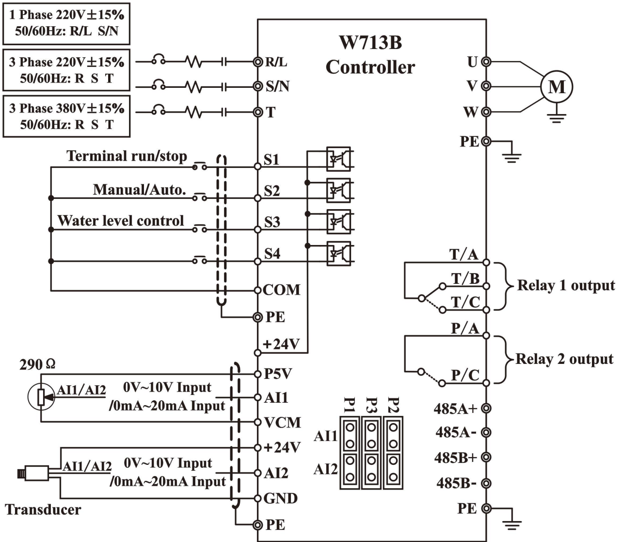
Figure 4.3.1 Wiring diagram
