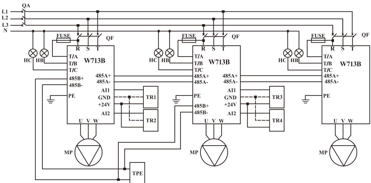
Figure8.2.2 Constant differential pressure control system wiring
