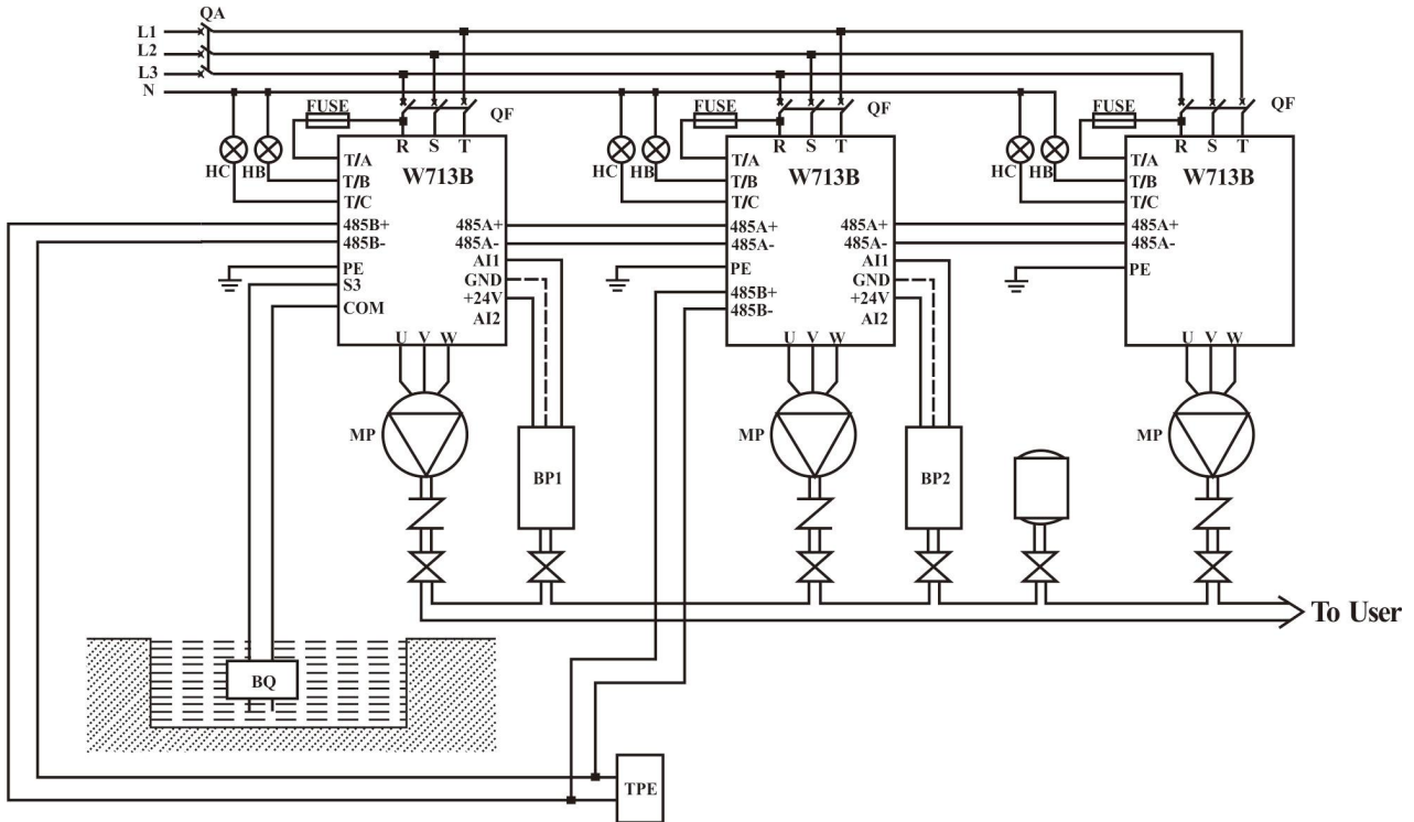
Figure8.3.3 Multi-pump linkage constant temperature water supply wiring
