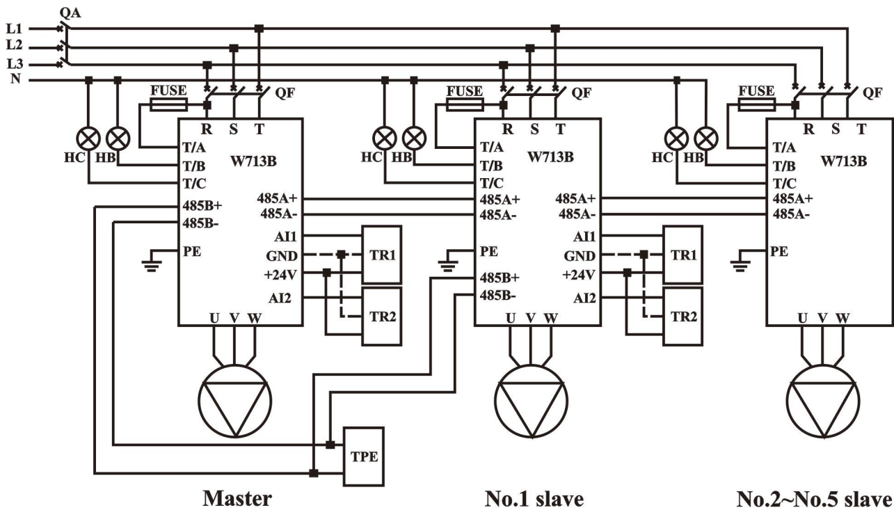
Figure 7.1.4 Multi-Pump water supply system wiring
