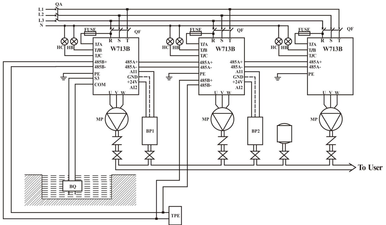
Figure 8.1.3 Multi-pump linkage constant pressure water supply wiring
