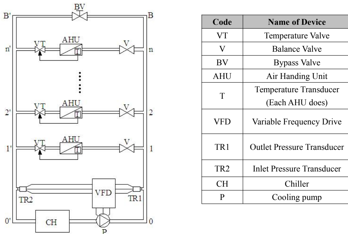
Figure8.2.1 Constant differential pressure control system
