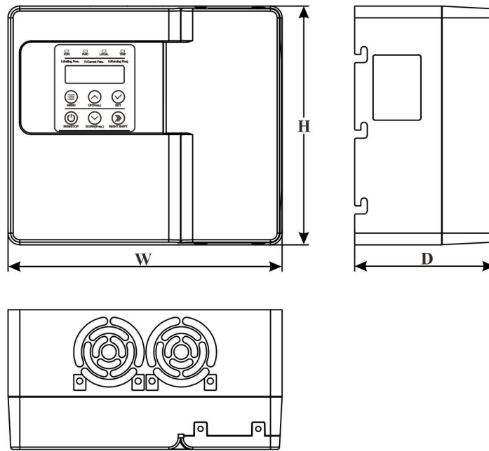
Figure 2.5.1 Dimension
